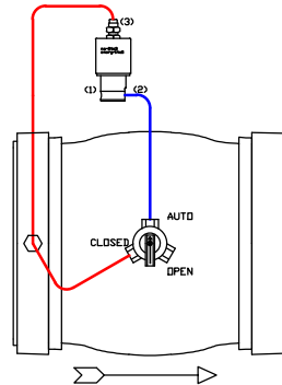
PRESSURE SUSTAINING 6000 SERIES PILOT AND CHECK VALVE
