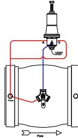
PRESSURE SUSTAINING/ REDUCING 6000 SERIES PILOT
