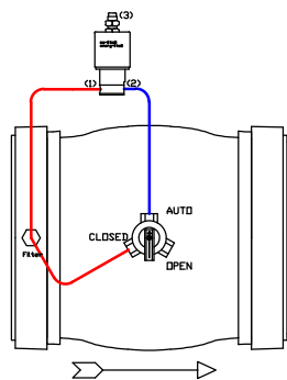
PRESSURE REDUCING & ELECTRIC ON/OFF 6000 SERIES PILOT AND CHECK VALVE
